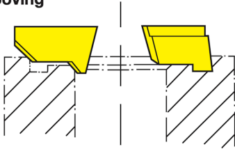
Facegrooving
