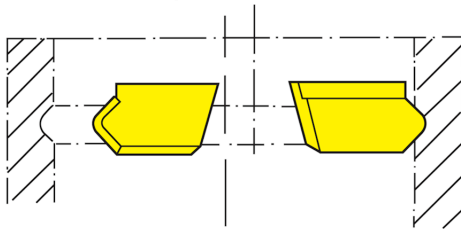
Groove milling by circular interpolation (inside and outside)
