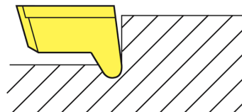
Axial undercut
